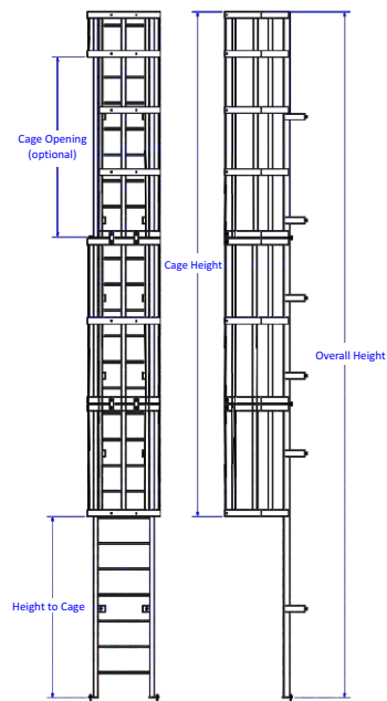
Caged Ladder
