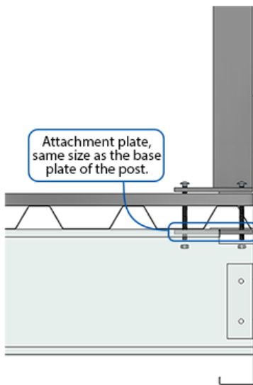
CONNECTION WITH EXISTING MEZZANINE (CORRUGATED STEEL DECK FLOORING)
