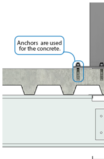
CONNECTION WITH EXISTING MEZZANINE (CONCRETE FLOORING)
