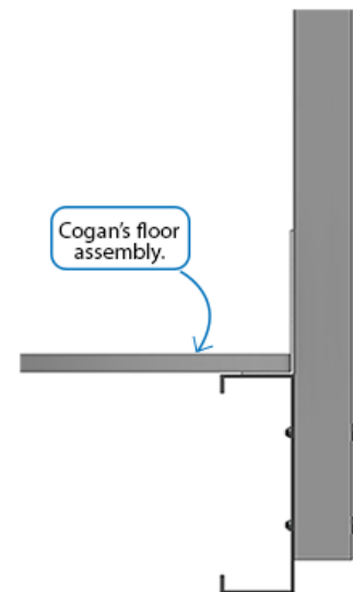
CONNECTION WITH COGAN'S MEZZANINE
