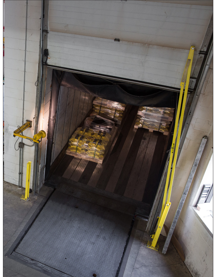
In the open position the gate stores to right to allow the trailer to be loaded or unloaded.
