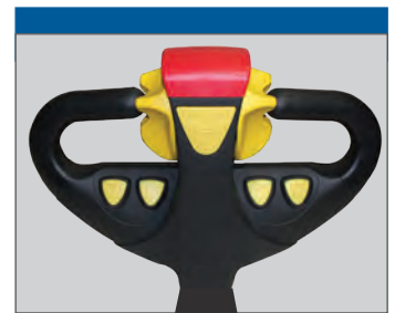
Ergonomic handle with comfort-grip controls and switch redundancy for left- or right-hand operation.
