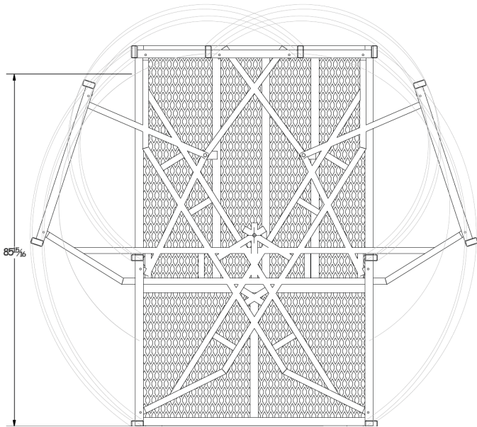
Pallet Drop Zone Gate swing path
