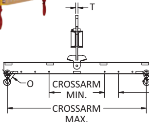
MODEL 27SD
