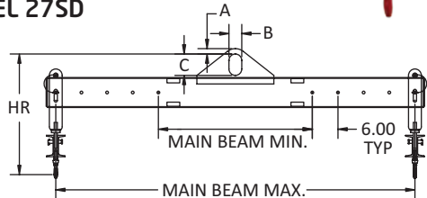
MODEL 27SD
