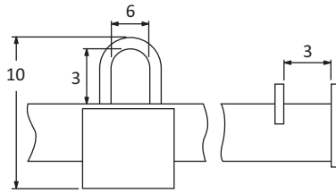
MODEL 27SL
