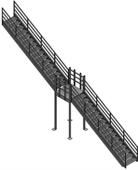
STRAIGHT STAIRCASE
