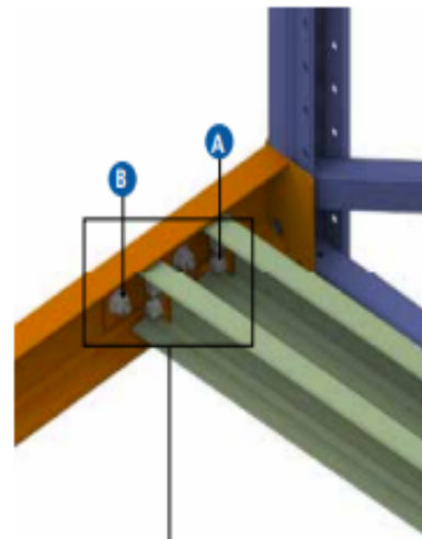
-3, 4 & 5 deep configuration assembly detail-
