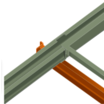
Push Back rail and interior/rear beam assembly
