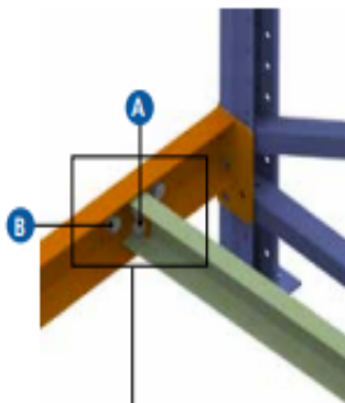
-2 deep configuration assembly detail-
