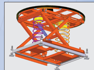
Leveling Feet
