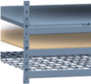
Steel beams designed for several decking types: steel, wire mesh and wood.
