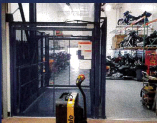
Motorcycle Lift – 21 Series Hydraulic VRC Transports motorcycles and parts between service and storage levels. 2,000 lbs. lifting capacity.
